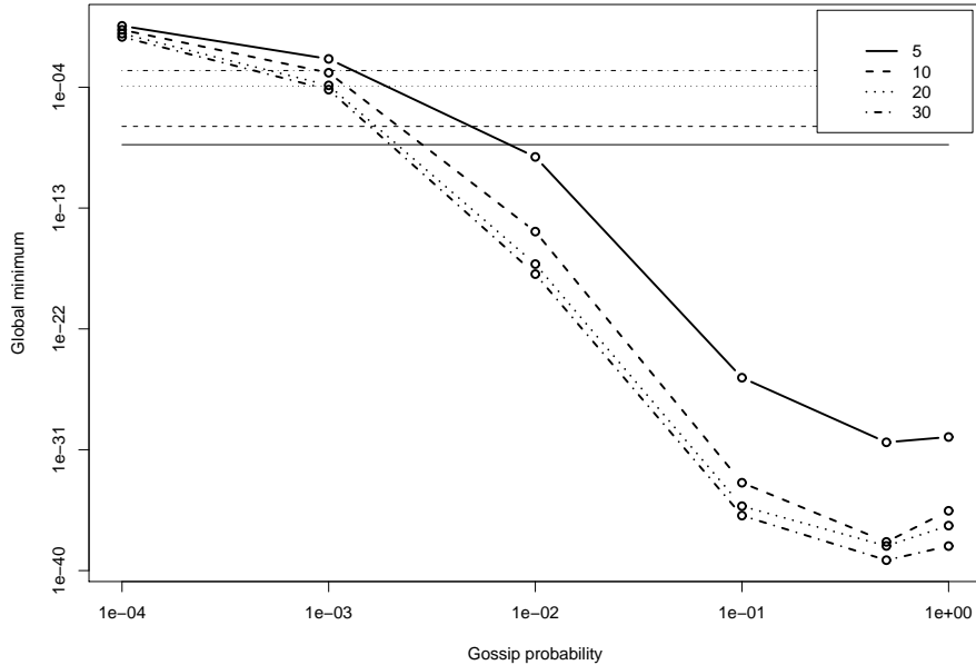
Figure 1: PSO with various message exchange probabilities; horizontal lines refer to the single-node scenario
