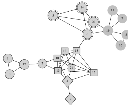
Figure 8: Graph-based representation of the network of contacts, as obtained from the real-world experimentation. An edge exists between any 2 vertexes if the corresponding persons have been in proximity for approximately 30 minutes per day.
