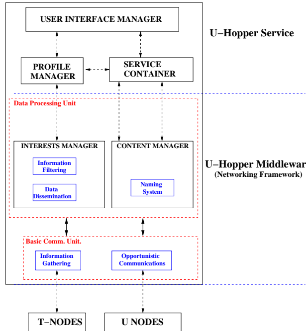
Figure 1: Block diagram and interconnections of the U'Hopper platform. In blue are reported the components of the BIONETS Serworks architecture, and their positioning inside the U'Hopper components.
